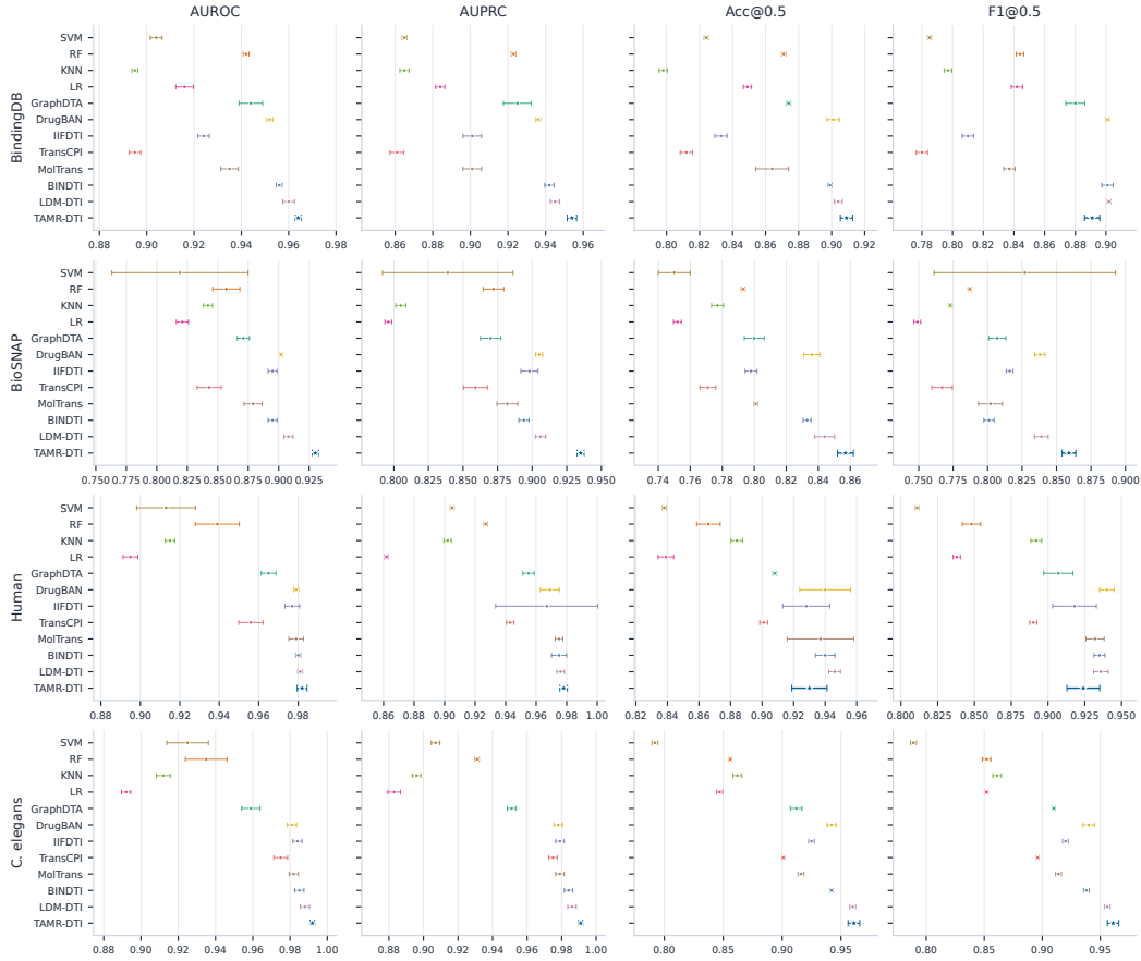
Figure 3: All-method uncertainty comparison on AUROC, AUPRC, Acc@0.5, and F1@0.5. Intervals are derived from mean and standard deviation summaries; TAMR-DTI intervals are computed from five local seeds.
