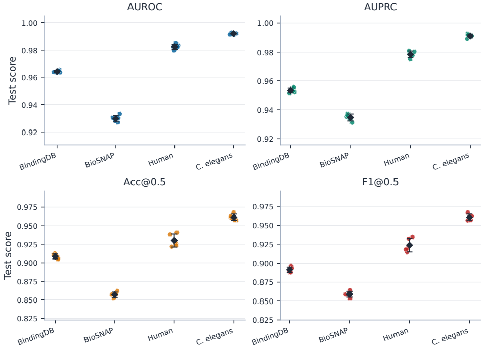
Figure 4: Five-seed stability of TAMR-DTI on the four benchmark datasets. Dots denote individual seeds 42, 43, 44, 45, and 46; diamonds denote seed means; and error bars denote one standard deviation. Acc@0.5 and F1@0.5 use the fixed threshold 0.5.
