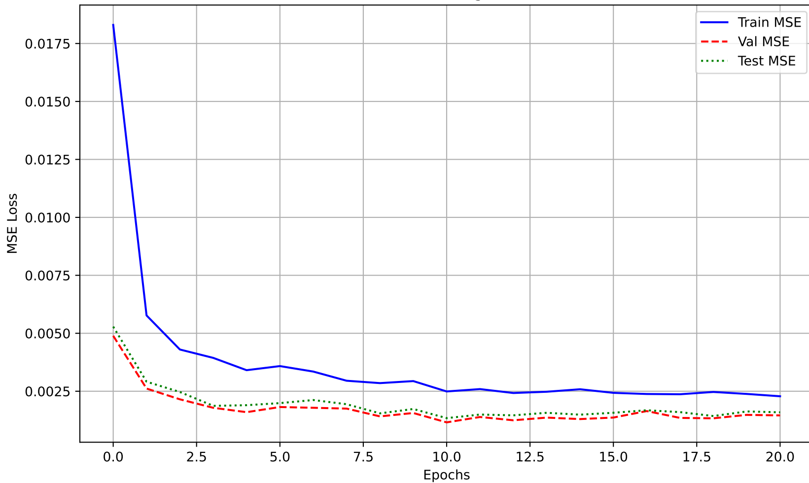
Phase 1: Pre-training Loss (MSE)
