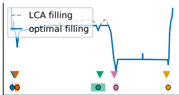
⑤ error 1.1%; \delta^* = 5.3 hPa (LCA 10.7)
