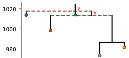
④ relax: flatten 2 weak merges (dashed)
