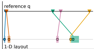
③ certificate \tau^* = 22\% , \tau_{free} = 0\%
