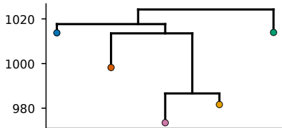
② merge tree T_t (join tree, hPa)
