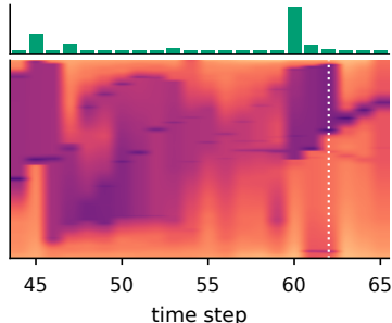
⑥ map with error strip
