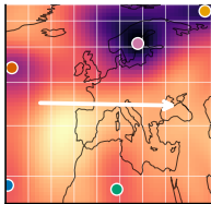
① field, extrema, reference direction
