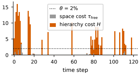
ERA5 2013/14: 30/124 with H > \theta
