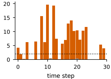
Wildfire 2019: 19/30 with H > \theta
