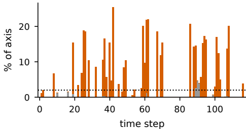
ERA5 1999/2000: 40/118 with H > \theta
