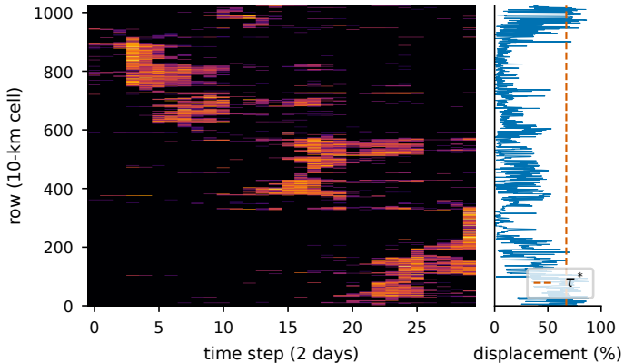
rows in OLO dendrogram order (fire time series)
