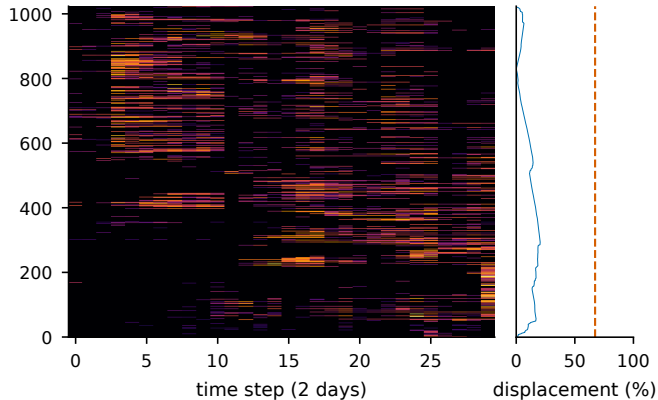
rows in geographic order (ignores dendrogram)
