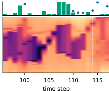
⑥ map with strips (error, \delta^* )
