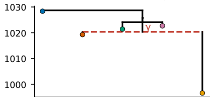
④ relax: flatten 1 weak merge (dashed)
