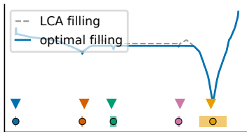
⑤ error 0.9%; \delta^* = 2.7 hPa (LCA 5.4)
