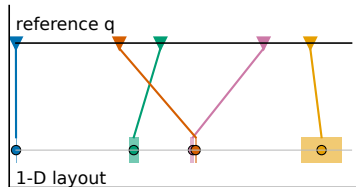
⑥ map with strips (error, \delta^* )
