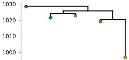
② merge tree T_t (join tree, hPa)
