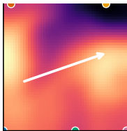
① field, extrema, reference direction
