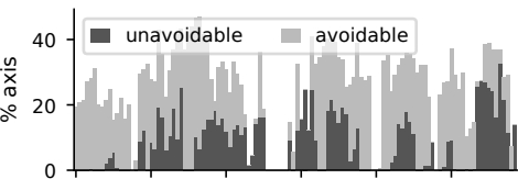
(a) ST-MTM: deviation of its order
