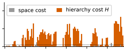
(b) Merge tree kept: certificate \tau^*
