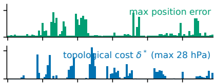
(c) Relaxed ( \kappa = 20\% ), optimal filling
