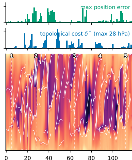
(c) Relaxed ( \kappa = 20\% ), optimal filling
