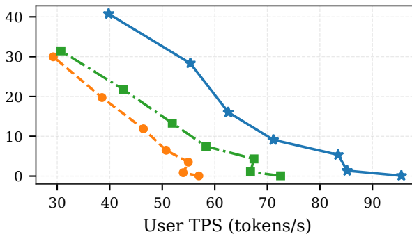
DeepSeek-V3 Decode
