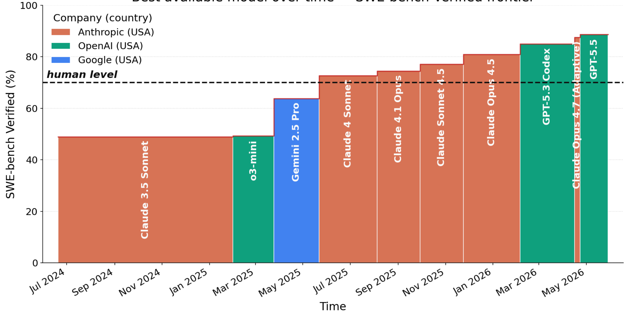
Best available model over time — SWE-bench Verified frontier
