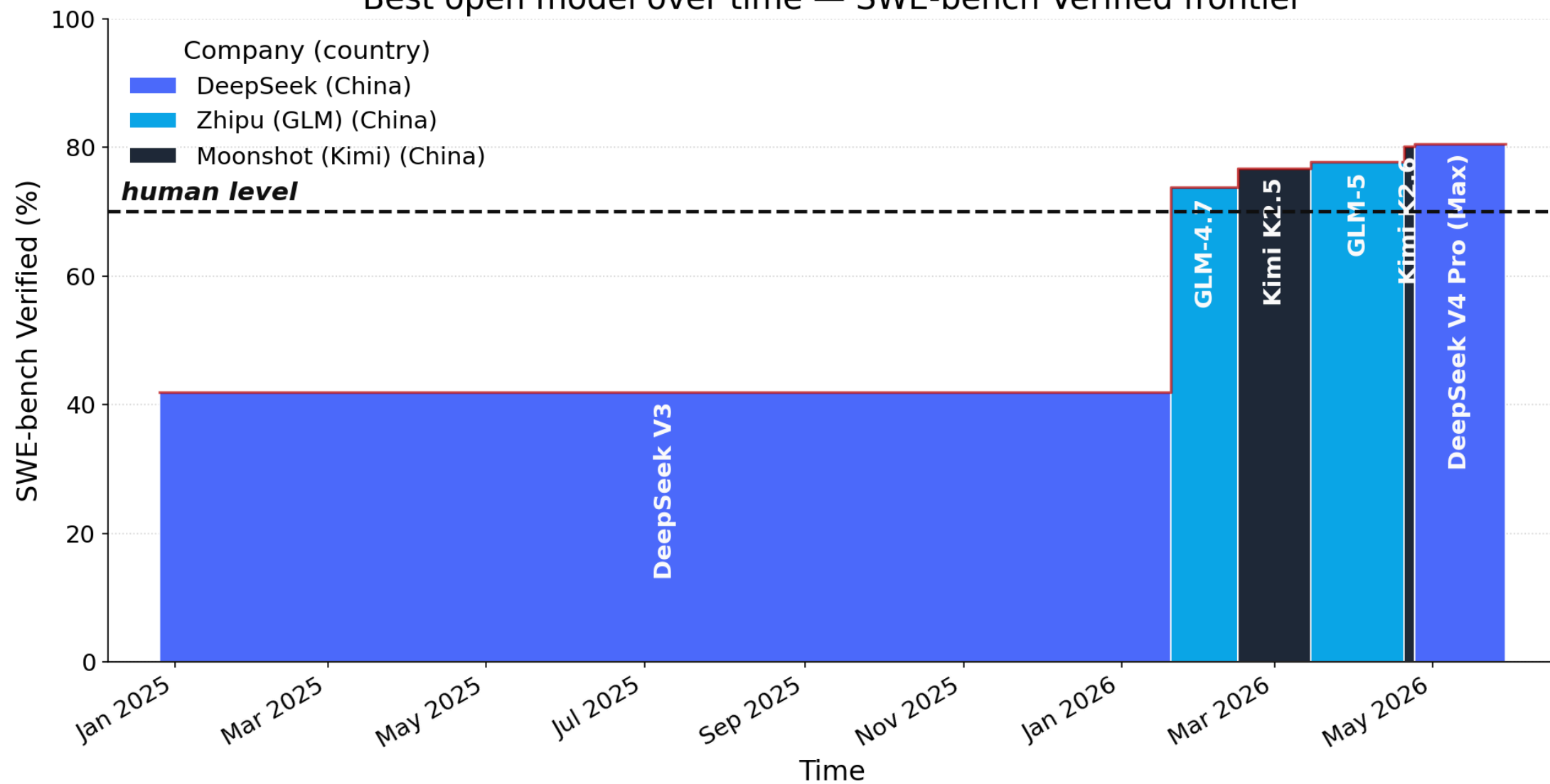
Best open model over time — SWE-bench Verified frontier
