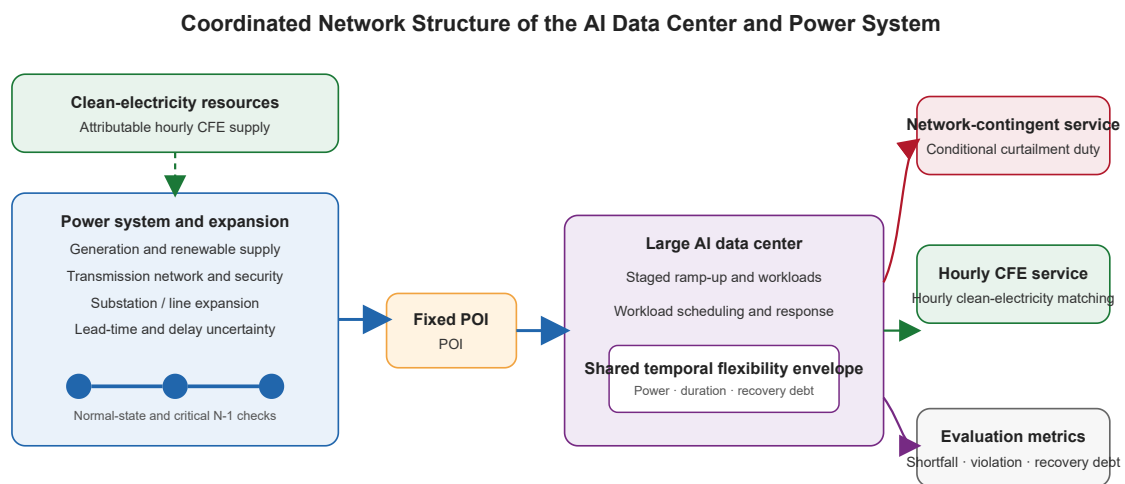
Figure 3. Coordinated network structure of the AI data center and power system.
