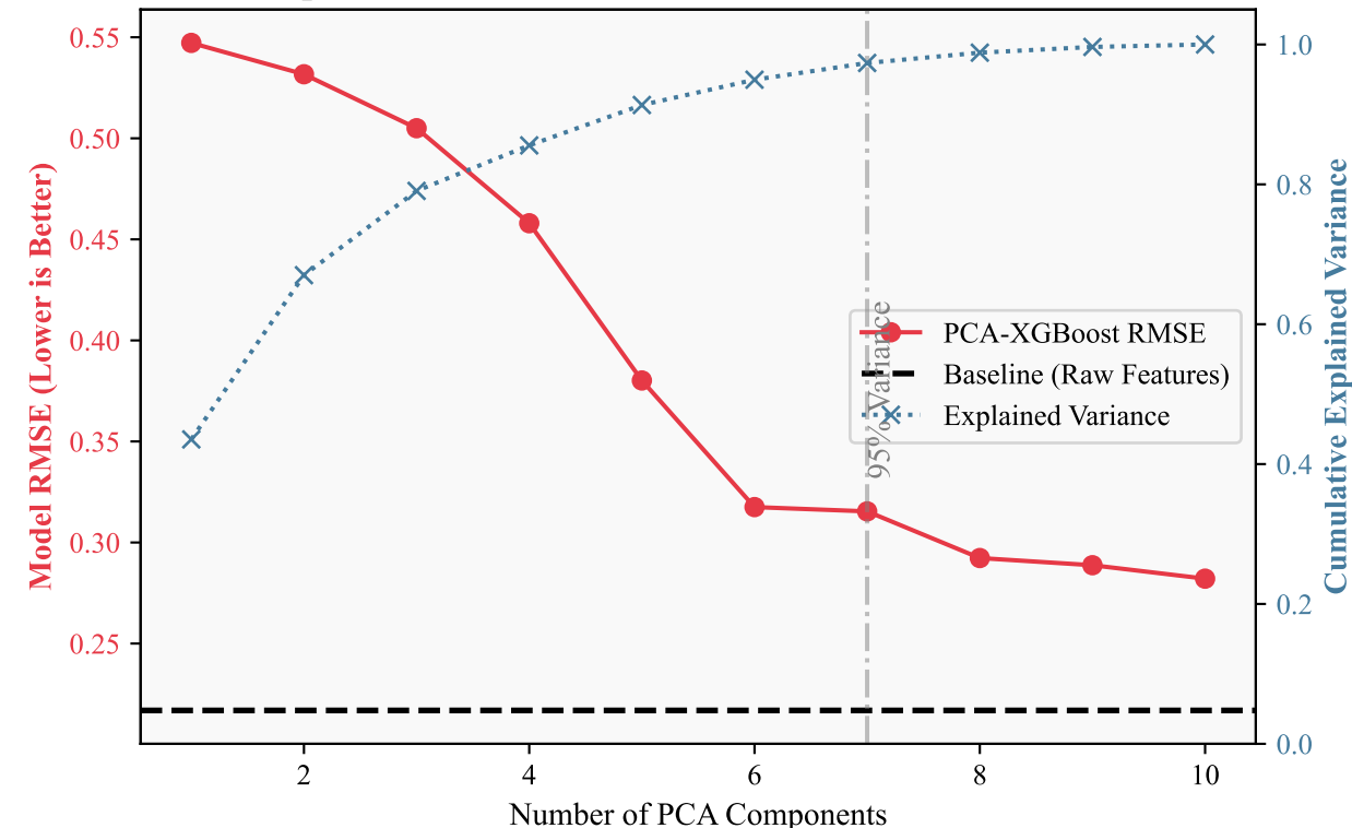
C. Impact of PCA Transformation on XGBoost Performance
