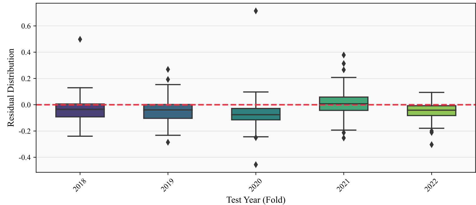
C. Residual Stability Over Time (Check for Temporal Bias)
