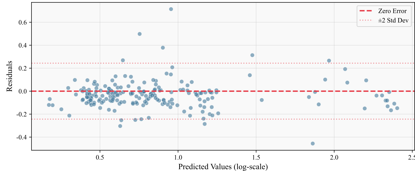
B. Residuals vs. Predicted Values (Check for Homoscedasticity)
