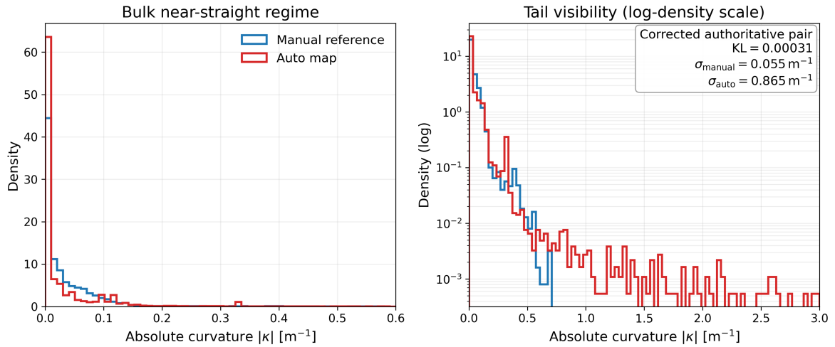
Figure 11: Corrected paramPoly3-aware curvature distributions for the authoritative Ingolstadt pair (manual Grid0828 reference versus contract-run auto XODR), with straight segments included exactly as in the authoritative run_11 measurement pair. The near-zero KL should be read together with the much larger auto-map spread and heavier high-curvature tail.
