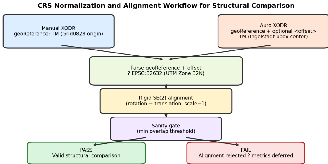
Figure 1: Coordinate normalization used for valid comparison between manual and automatically generated OpenDRIVE maps. Both sources are parsed (geoReference and optional offset), projected to a canonical CRS (EPSG:32632), and then aligned using a rigid SE(2) transform with a sanity gate.
