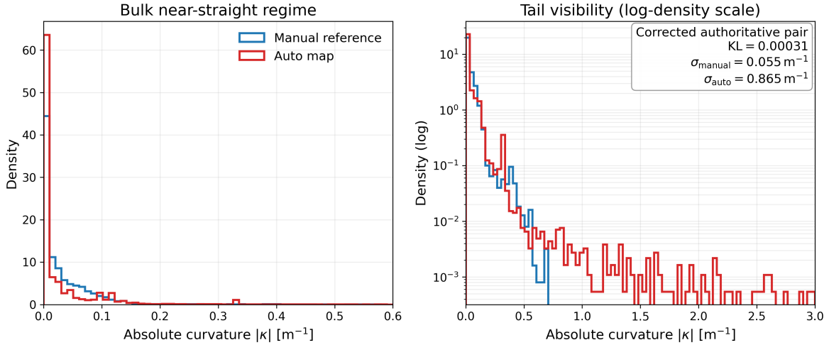
Figure 13: Corrected paramPoly3-aware curvature distributions for the authoritative Ingolstadt pair (manual Grid0828 reference versus contract-run auto XODR), with straight segments included exactly as in the authoritative run_11 measurement pair. The near-zero KL should be read together with the much larger auto-map spread and heavier high-curvature tail.
