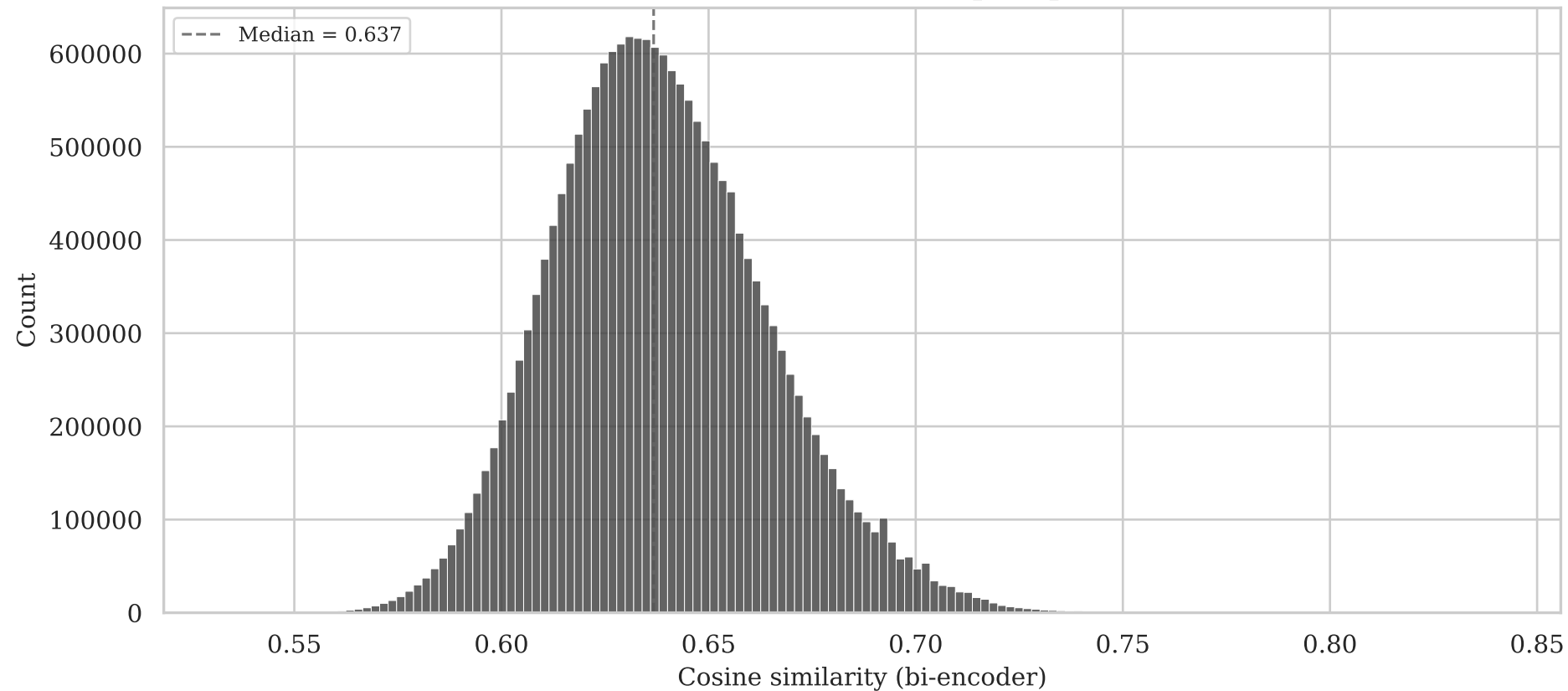
Bi-encoder score distribution — Full BDC retrieval corpus (n = 19,125,540 candidates, top-20 per chunk)
