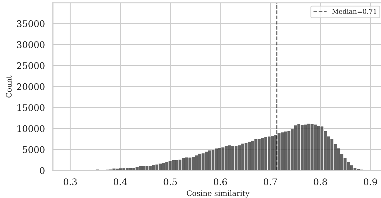
LaBERTa (bi-encoder) — score distribution
