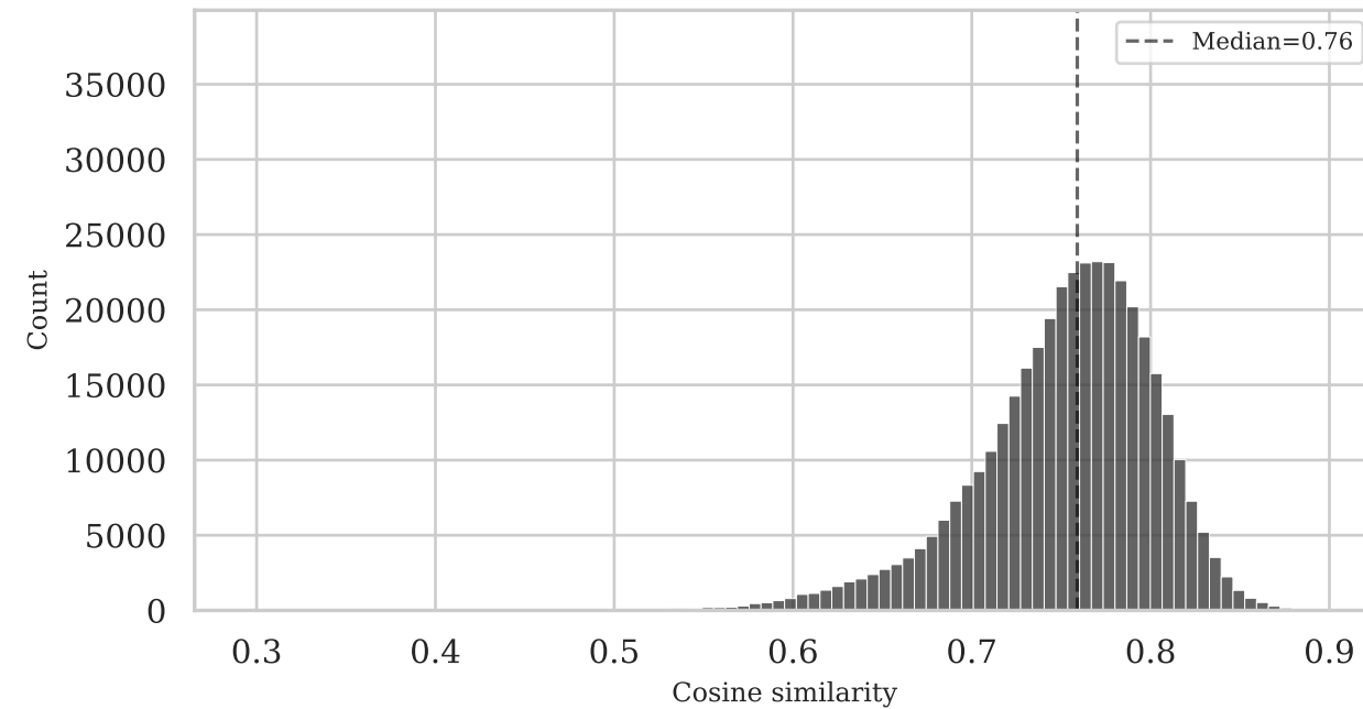
SPhilBERTa-intertext (bi-encoder) — score distribution
