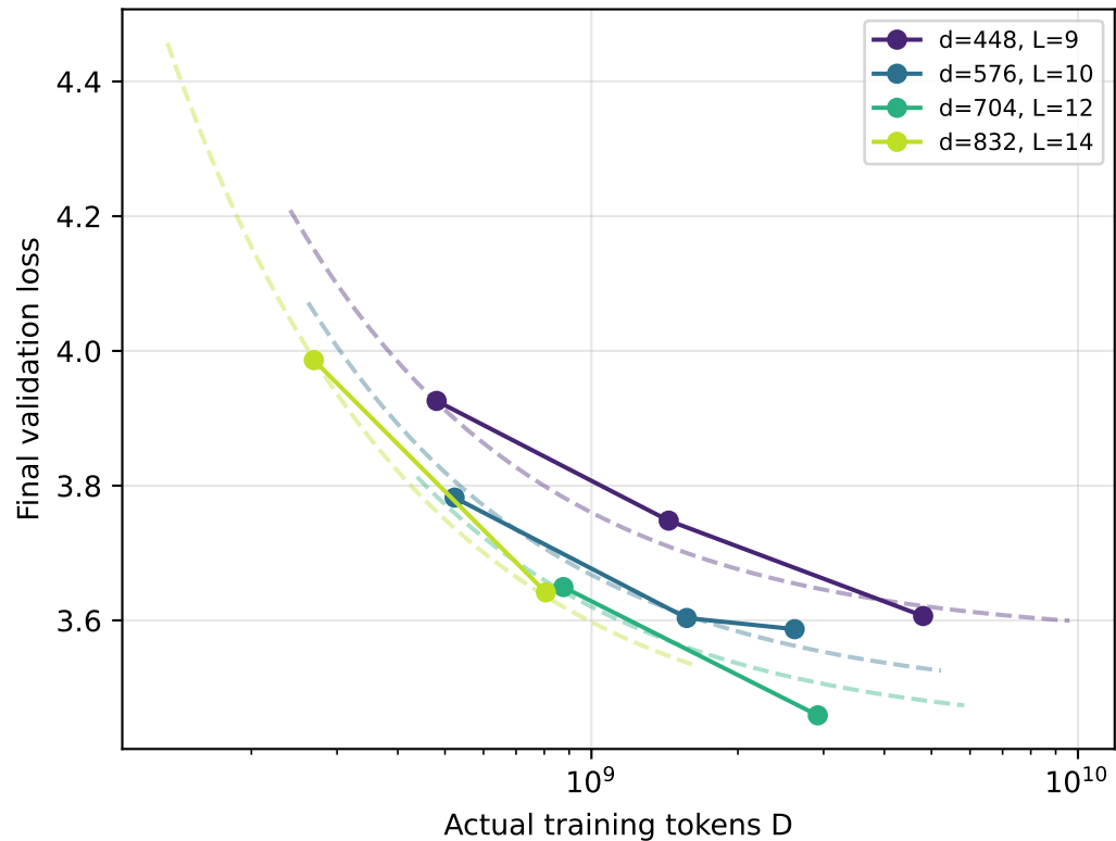
Loss vs D per family
