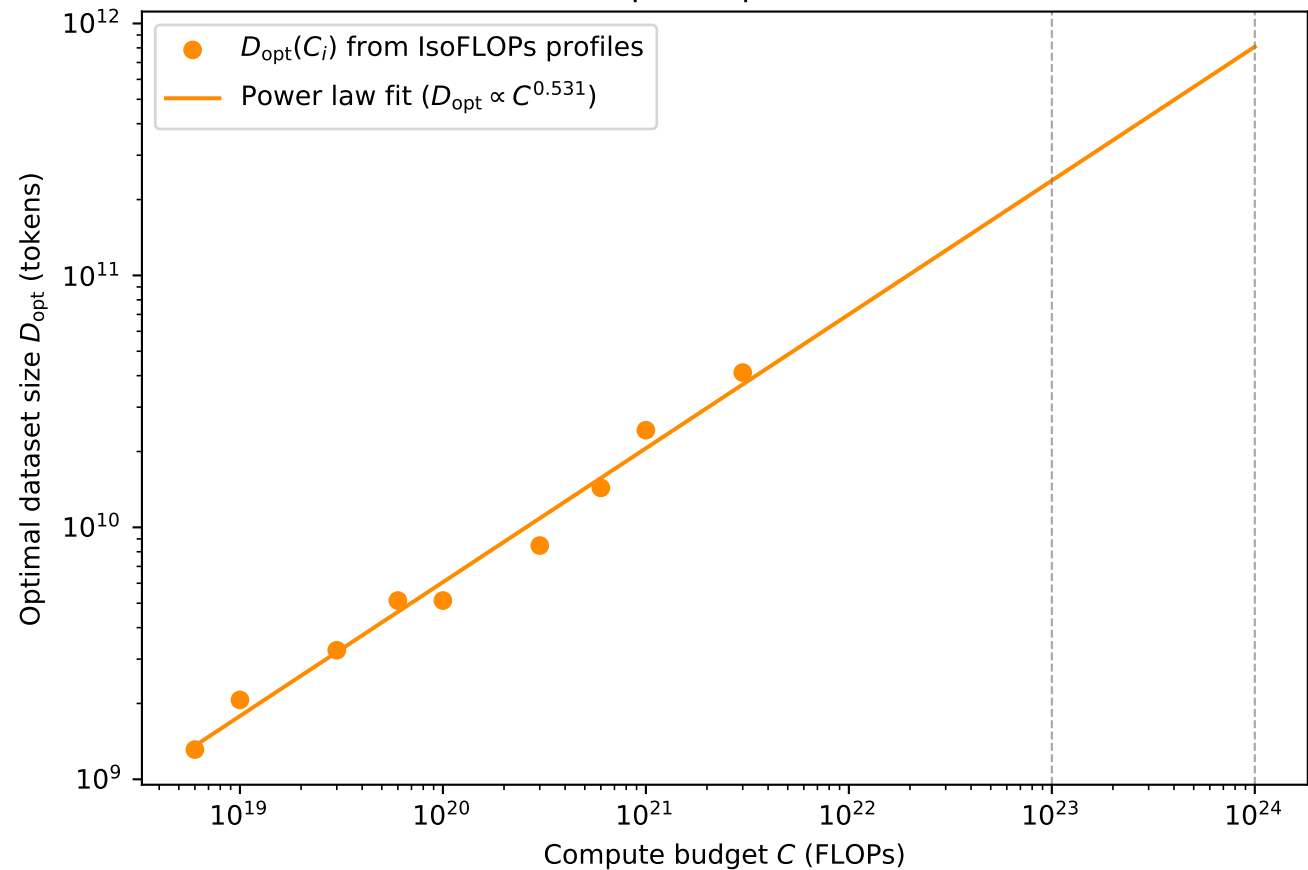
IsoFLOPs: Compute-Optimal Dataset Size
