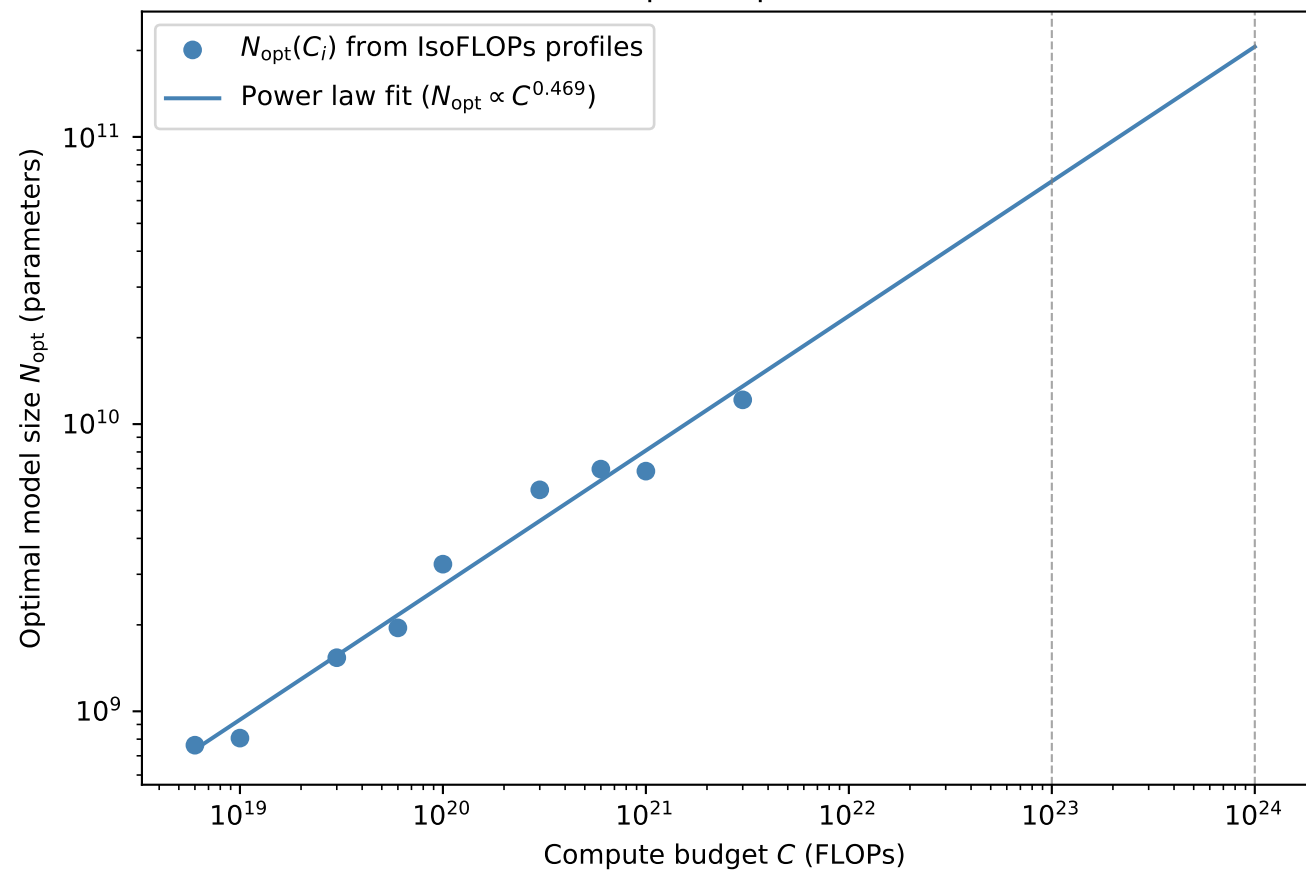
IsoFLOPs: Compute-Optimal Model Size
