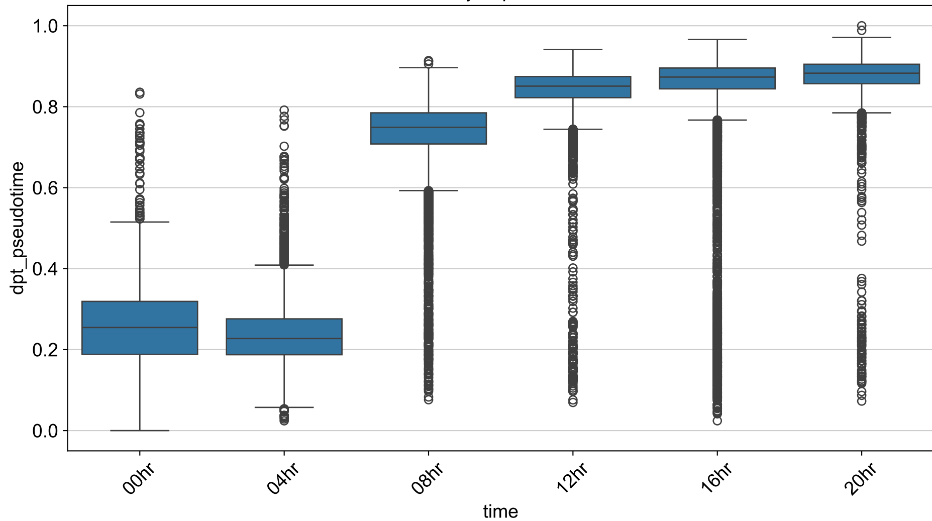
DPT Pseudotime by Experimental Time Points
