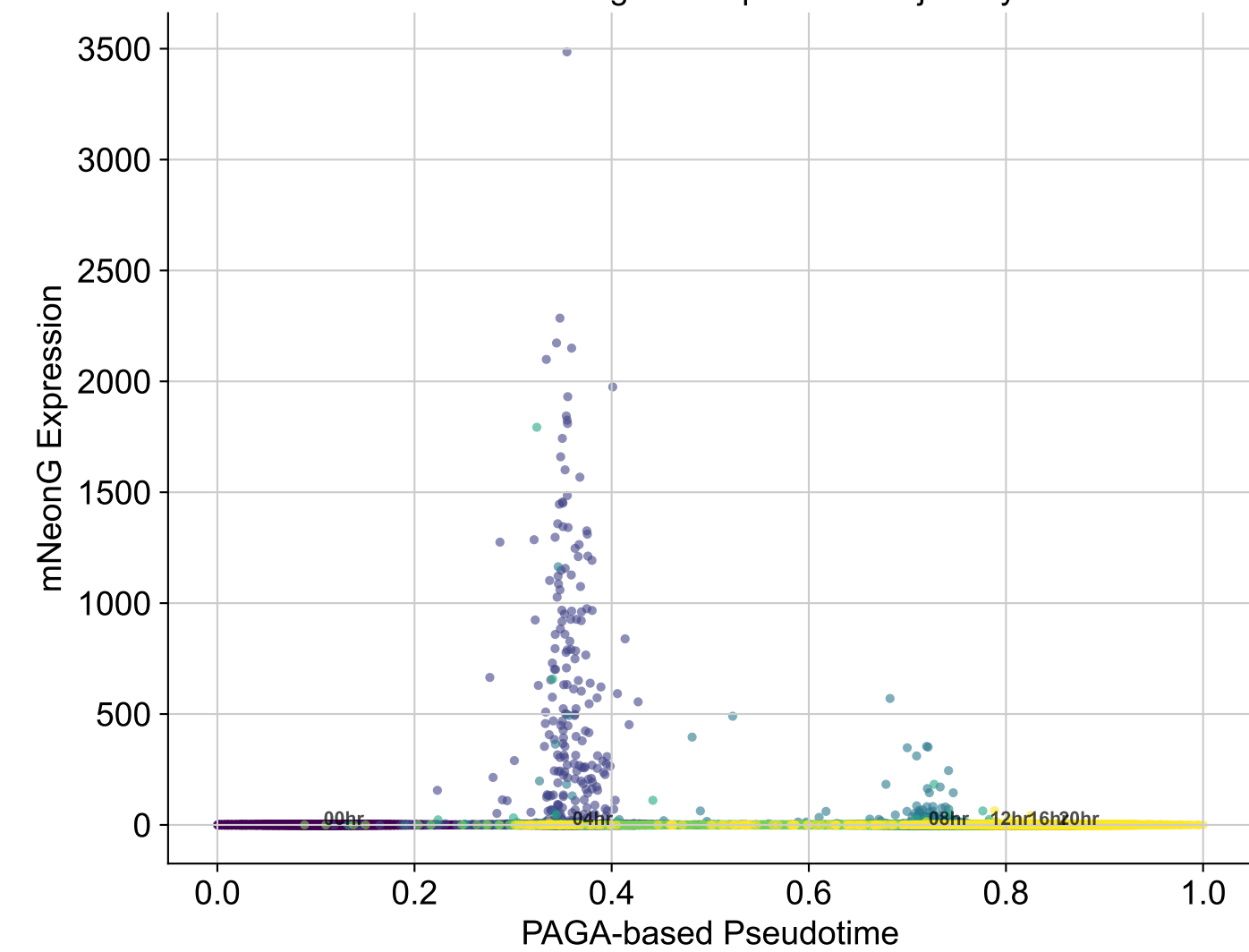
mNeonG along Developmental Trajectory
