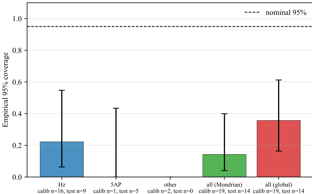
Scaffold-conditional (Mondrian) 95% conformal coverage (95% Wilson CIs)
