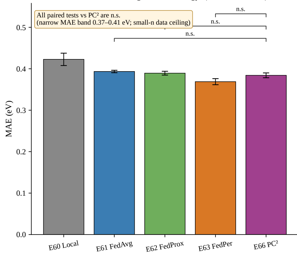
Client C — hole reorganization energy (n = 53, LOOCV)
