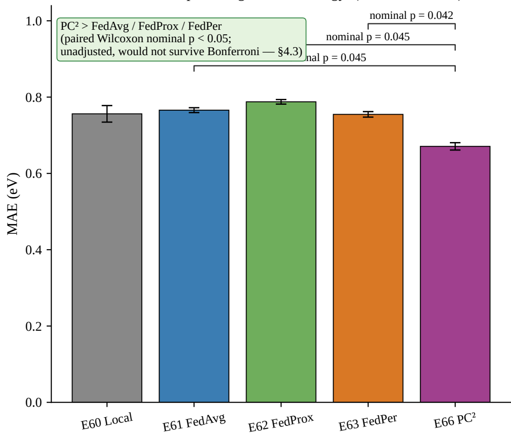
Client C — triplet reorganization energy (n = 49, LOOCV)
