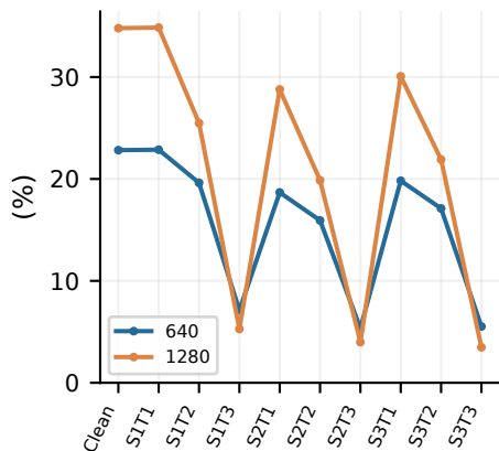
YOLO26s | All conditions: AP
