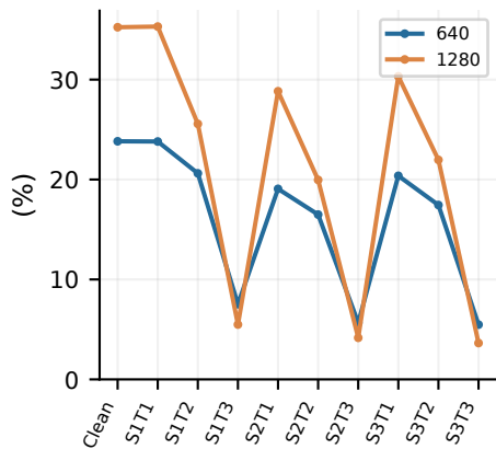
YOLO26s | All conditions: AP
