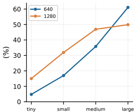
YOLOv8s | CLEAN: size AP
