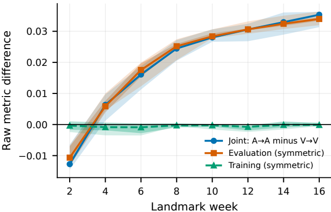
(a) ROC-AUC decomposition
