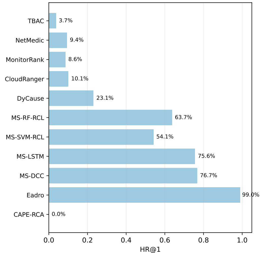
Eadro-TT
