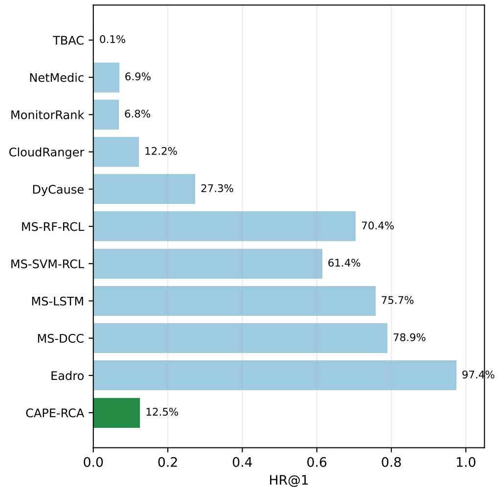
Eadro-SN
