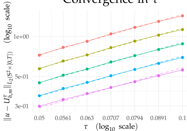
Convergence in \tau
