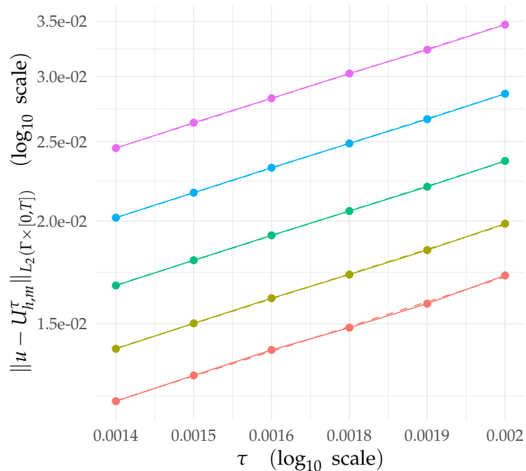
Convergence in \tau
