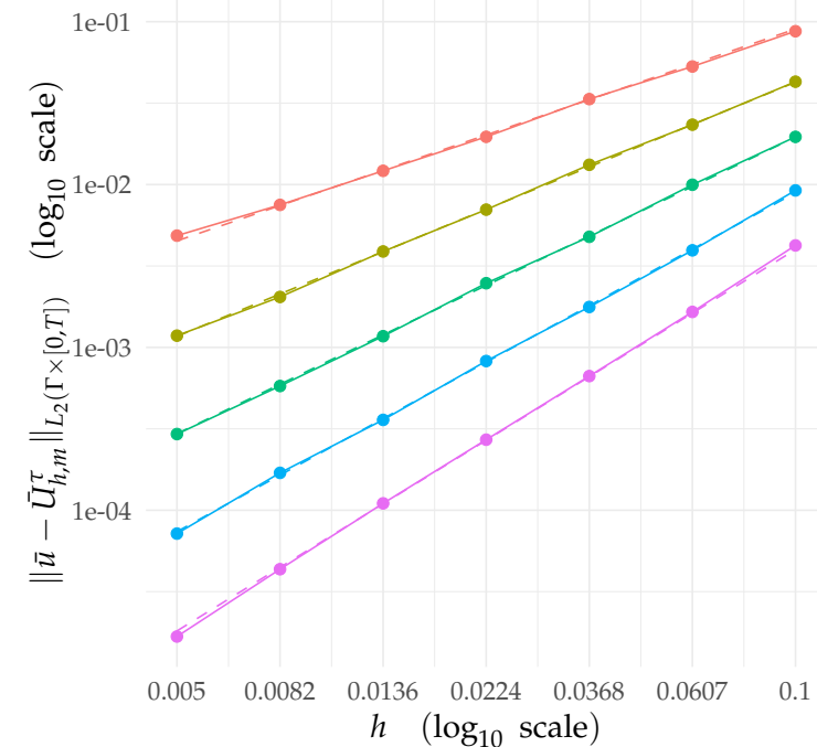
Convergence in h
