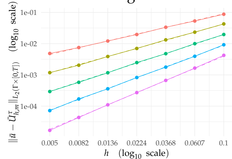
Convergence in h
