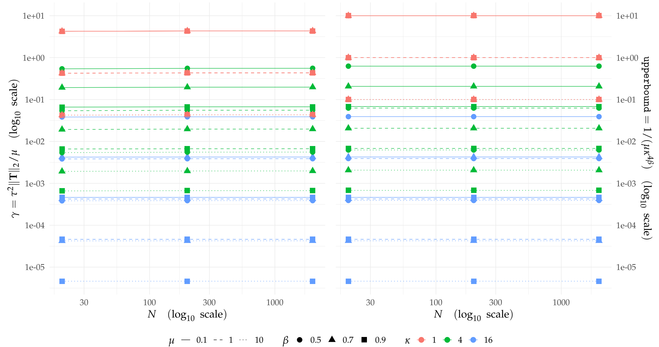
Contraction constant \gamma = \tau^2 \|\mathbf{T}\|_2 / \mu and its upper bound \text{upperbound} = 1 / (\mu \kappa^{4\beta})
