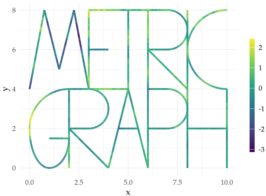
Simulated non-stationary process
