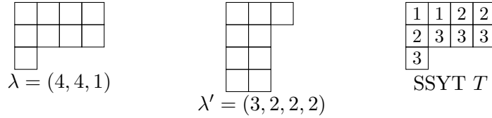
Figure 2: The partition \lambda = (4, 4, 1) (left), its conjugate \lambda' = (3, 2, 2, 2) obtained by reflecting across the main diagonal (middle), and a semistandard Young tableau T of shape \lambda with entries in \{1, \dots, n\} , n = 3 (right): rows weakly increase left to right, columns strictly increase top to bottom. The cells filled with a given entry k form a horizontal strip (at most one per column), so T records the horizontal-strip interlacing sequence \emptyset \prec (2) \prec (4, 1) \prec (4, 4, 1) . The weight of T is x^{\text{wt}(T)} = x_1^2 x_2^3 x_3^4 , and s_\lambda = \sum_T x^{\text{wt}(T)} is the sum of weights over all semistandard tableaux.
