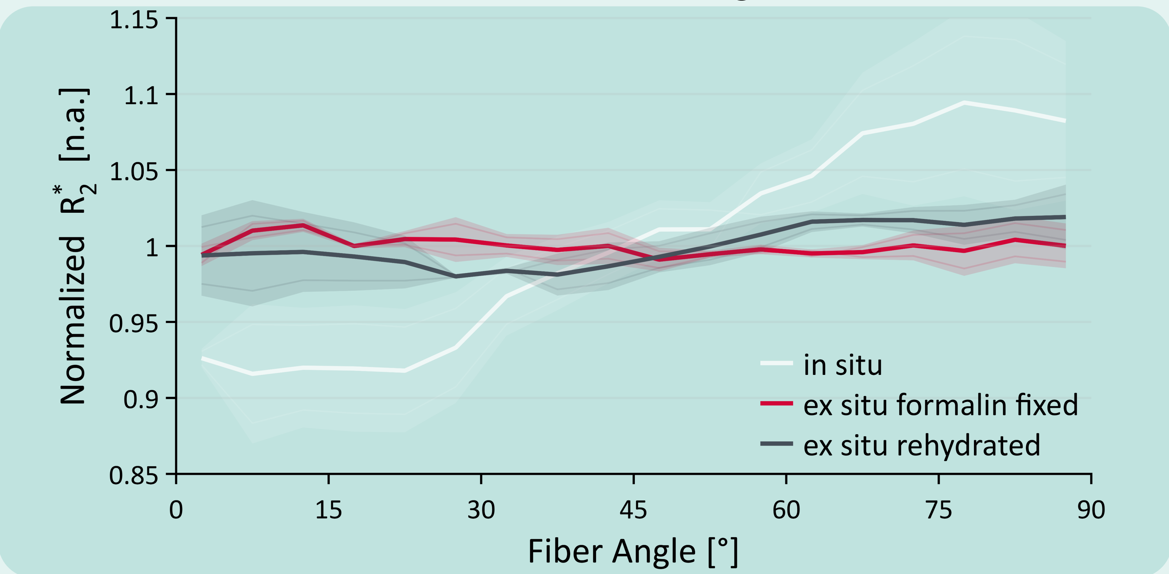
Figure 1: Normalized R_2^* values across the three tissue conditions over the calculated tissue fiber angle.
