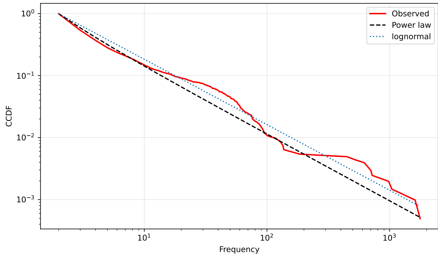
BPIC14 CCDF
