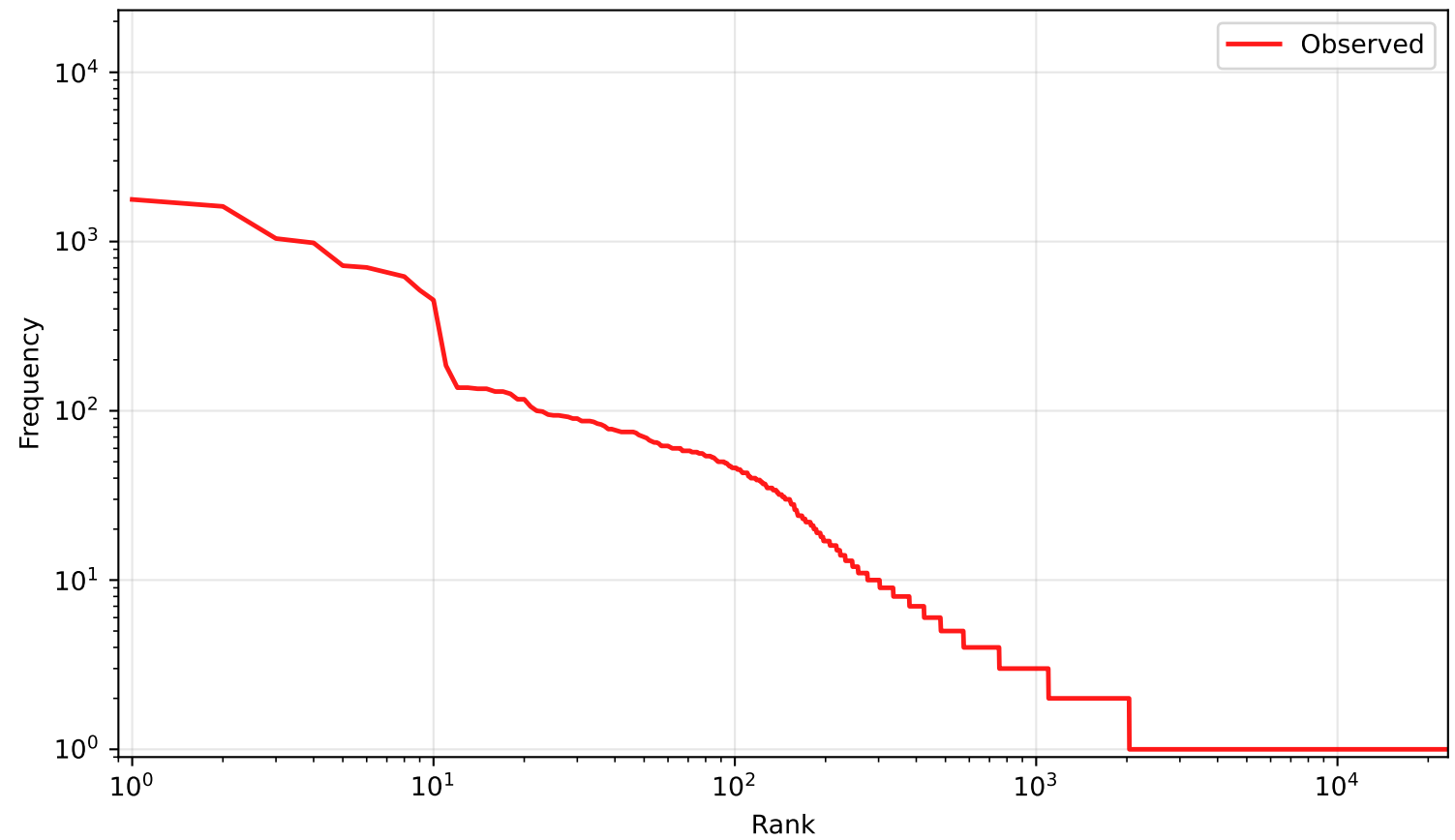
BPIC14 RFC
