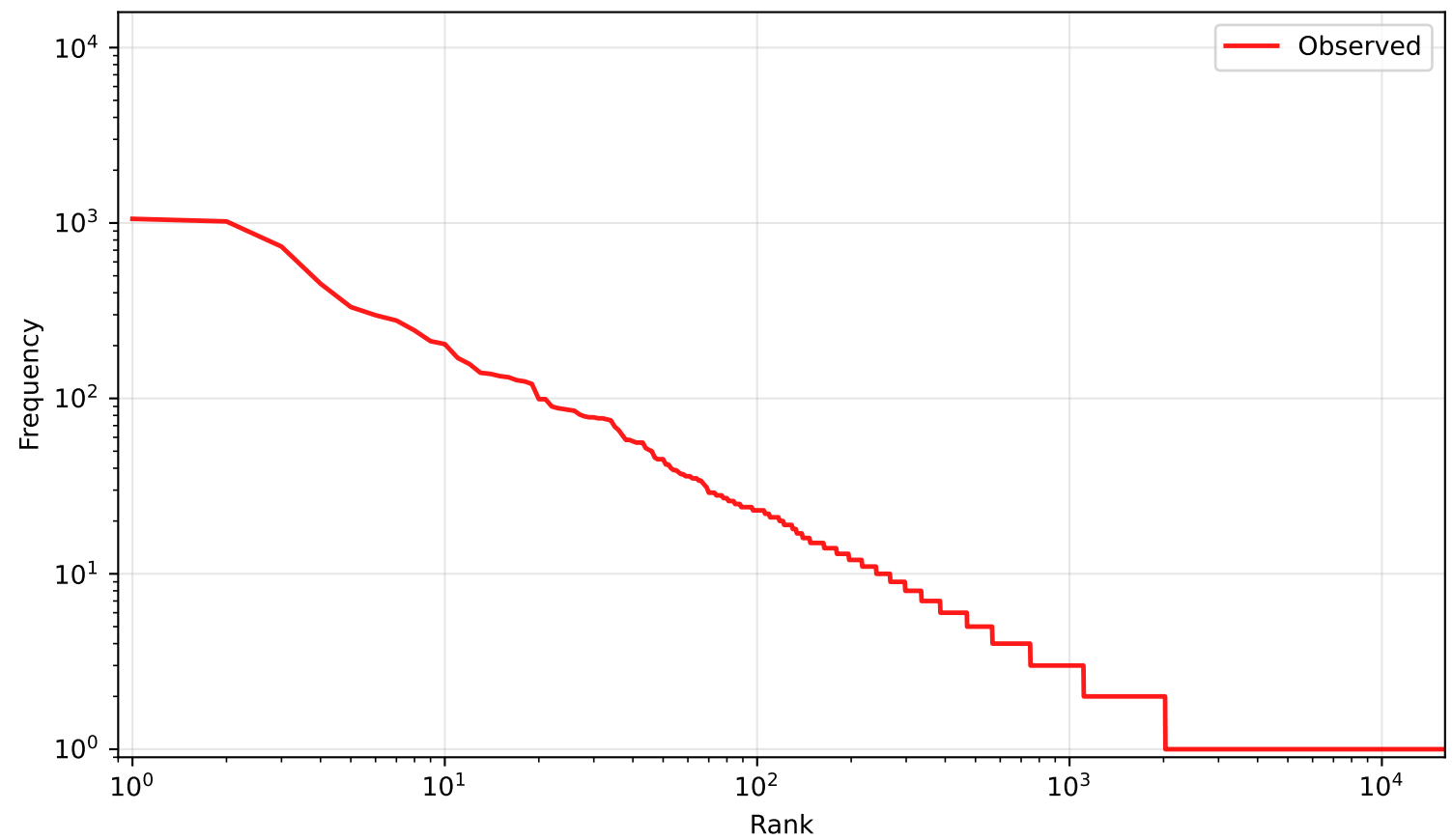
BPIC17 RFC
