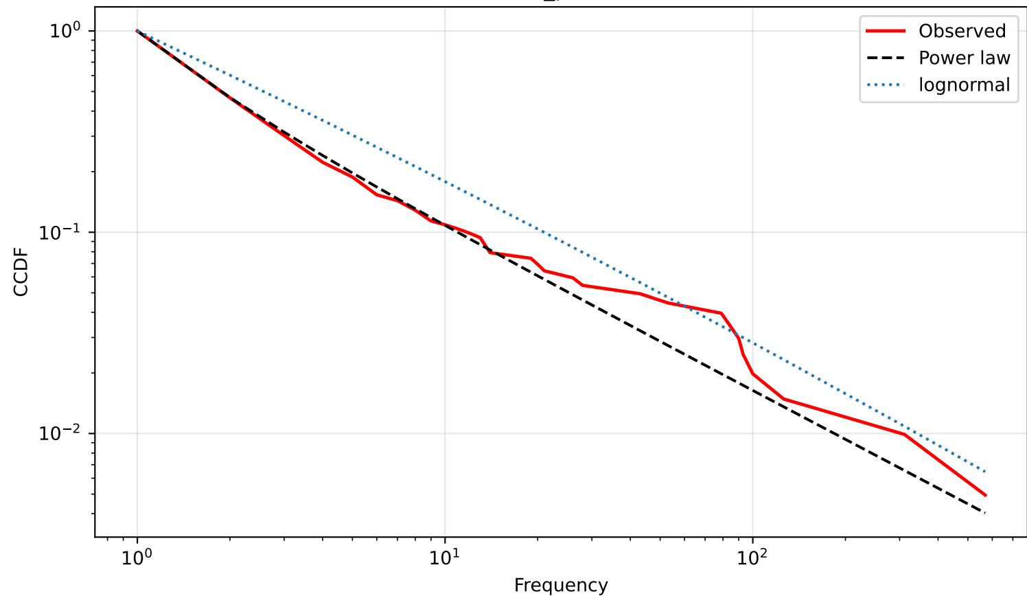
BPIC20_ptc CCDF
