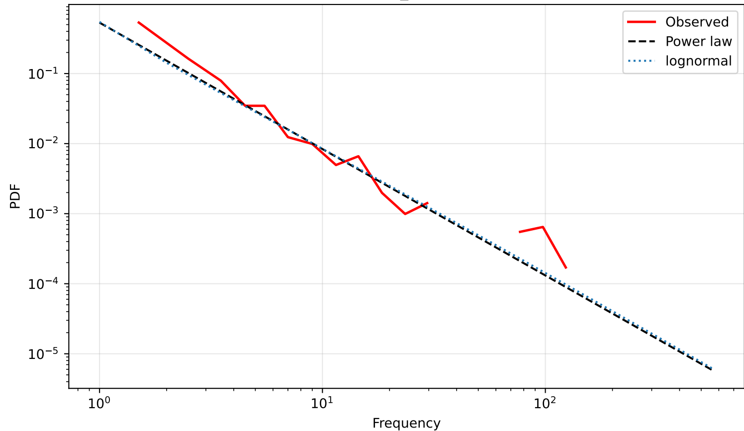
BPIC20_ptc PDF
