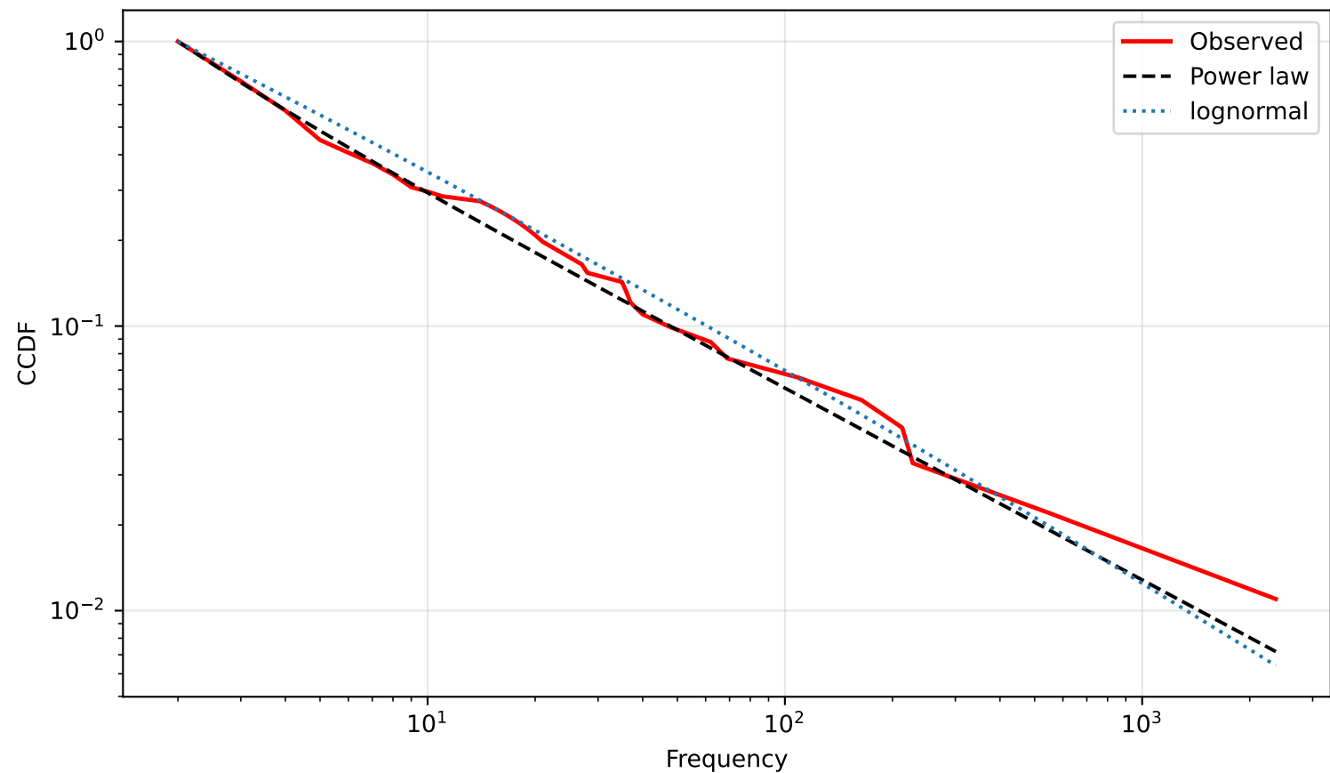
ITHD CCDF
