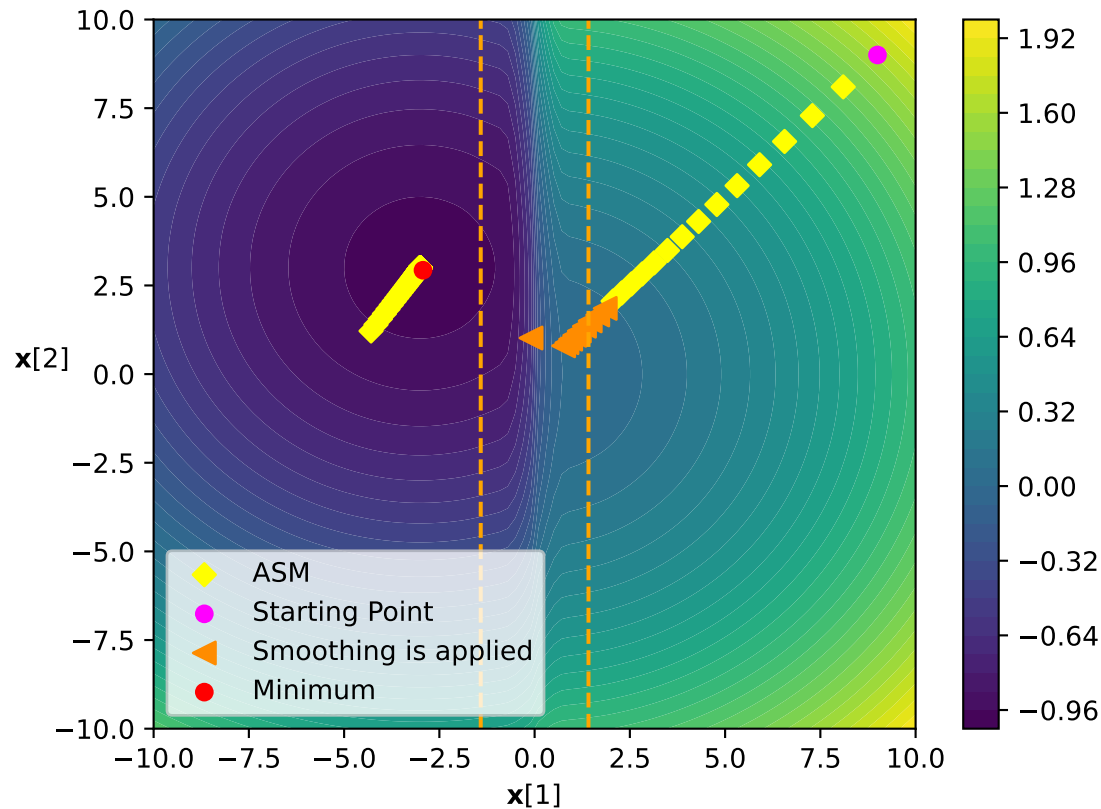
Landscape of \mathcal{F} and Optimization Steps
