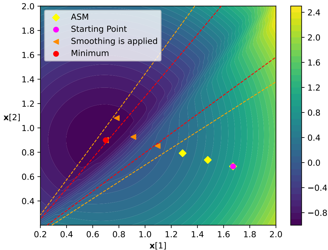
Landscape of \mathcal{F} and Optimization Steps
