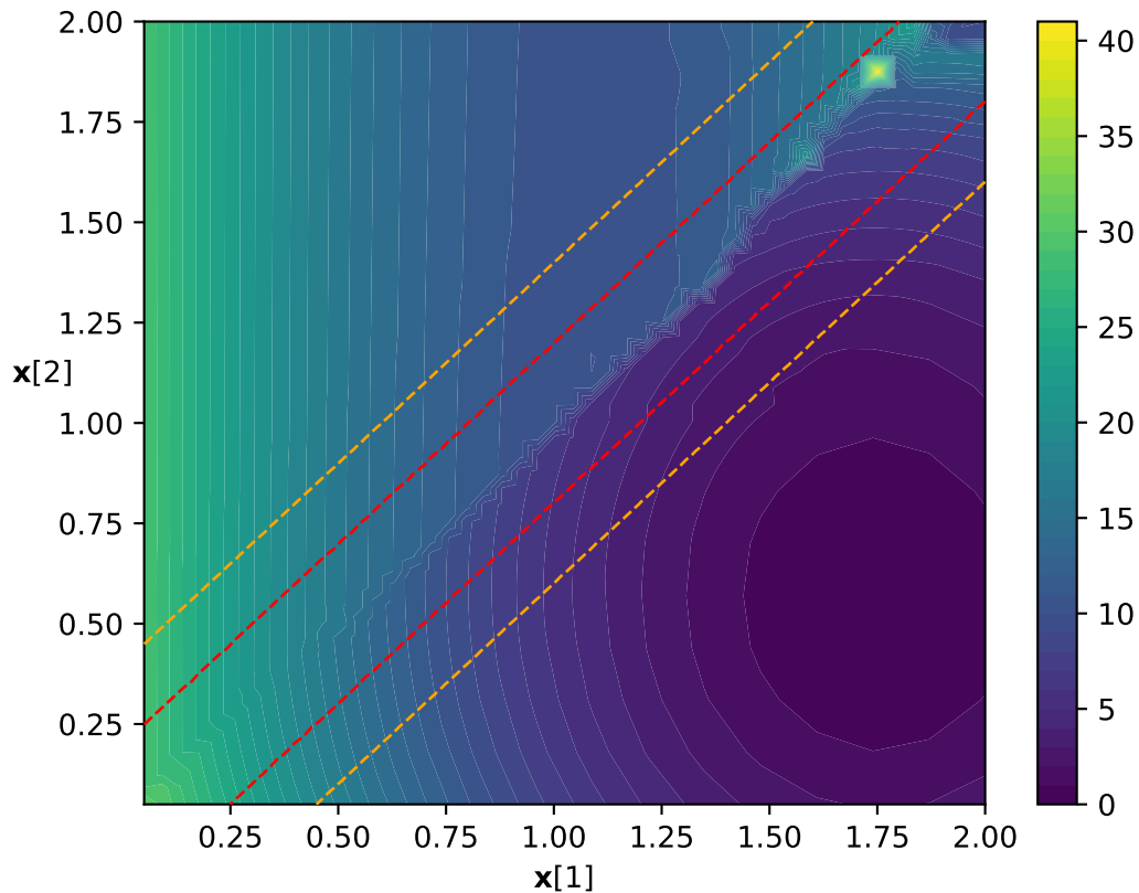
Landscape of energy diff all
