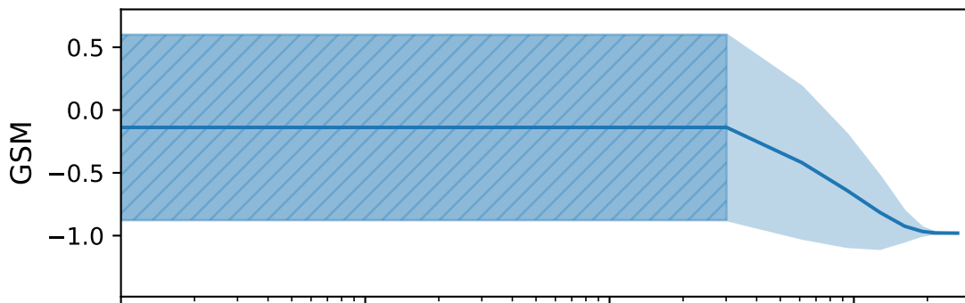
Mean and Standard Deviation in Objective Value for 128 random runs
