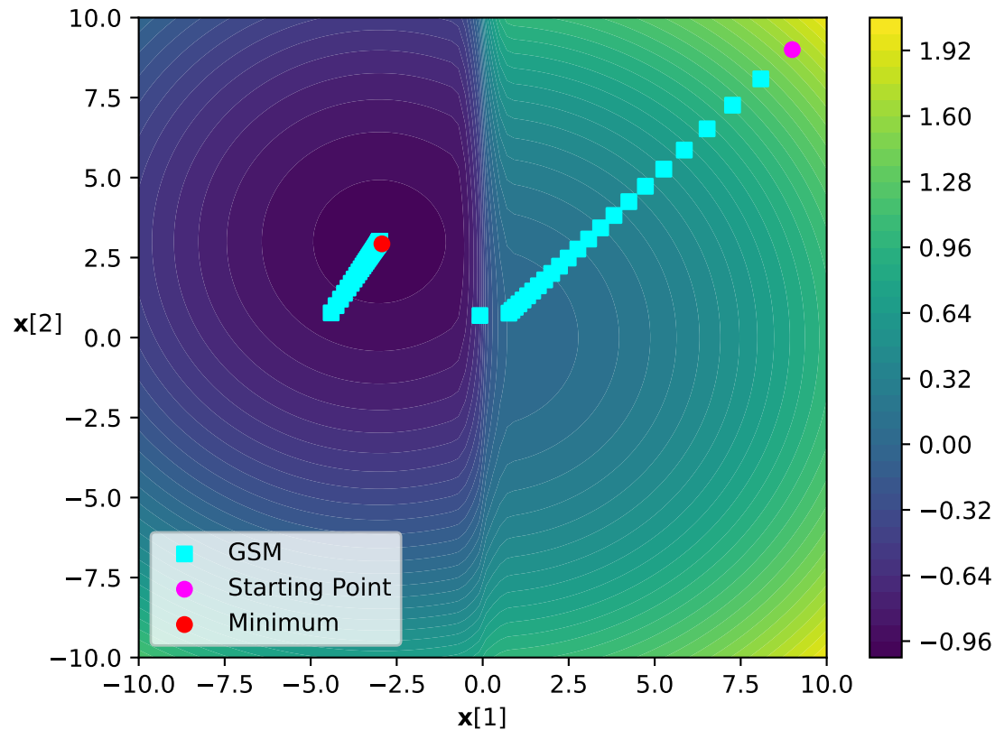
Landscape of F and Optimization Steps
