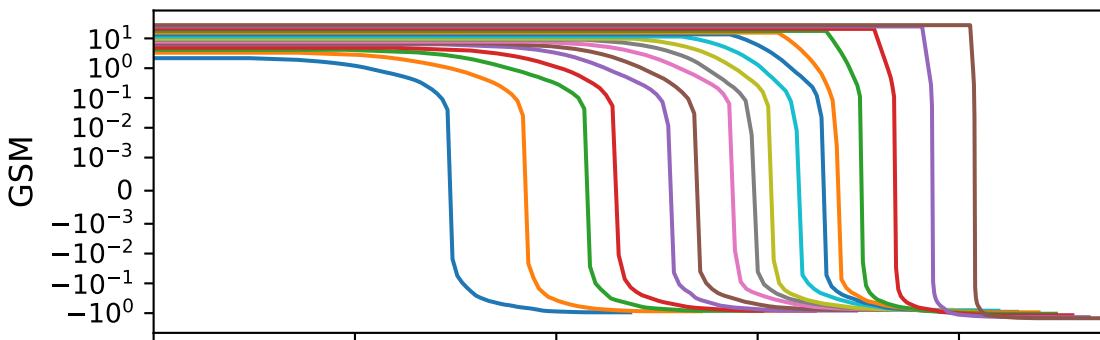
Mean Objective Value for 100 random runs with increasing dimension
