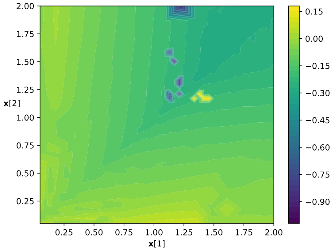
Landscape of eigs1
