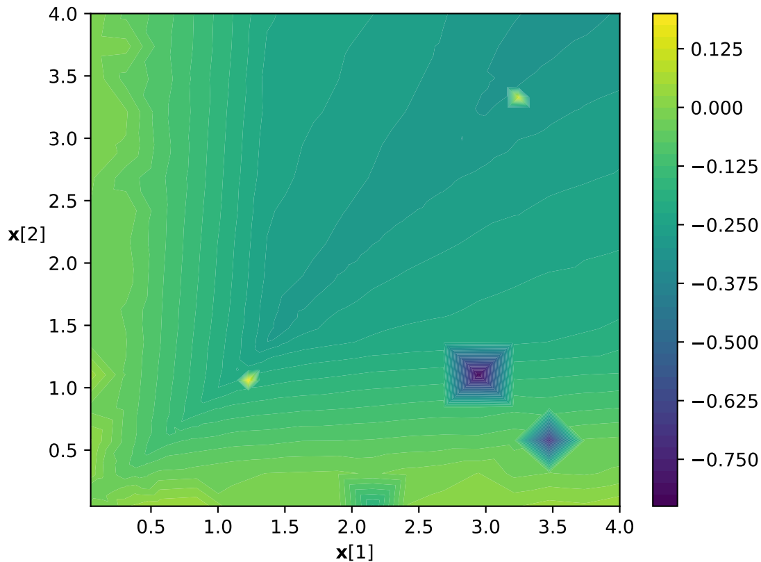
Landscape of eig1
