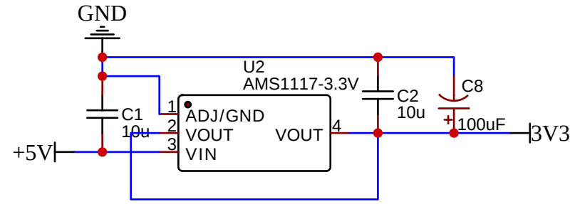
5V转3V
