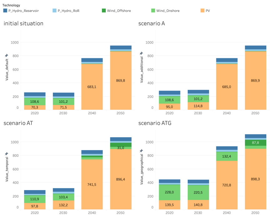
Figure B 4: Total capacity of RE in GW across the different scenarios
