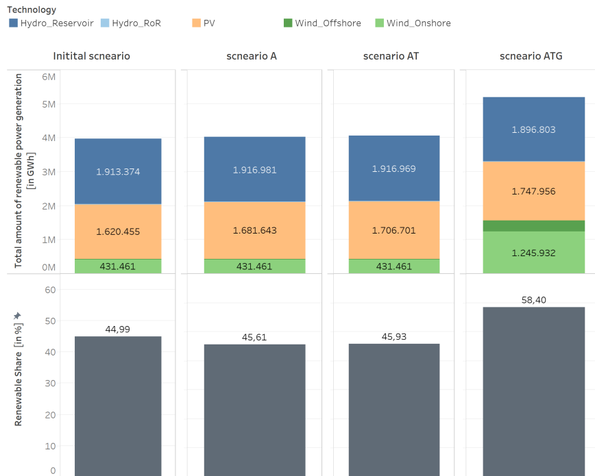
Figure B 6: Renewable Share and total amount of renewable power generation
