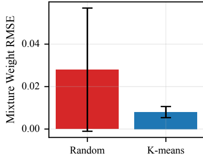
Mixture Weight RMSE
