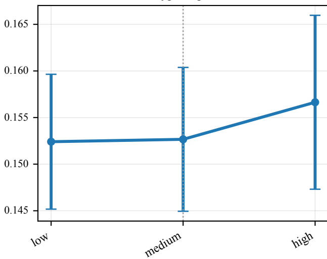
Archetype Separation
