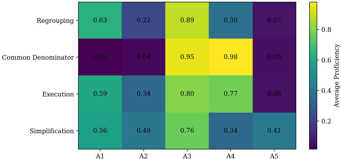
MoLA Archetype Alignment with Tatsuoka Rule Families
