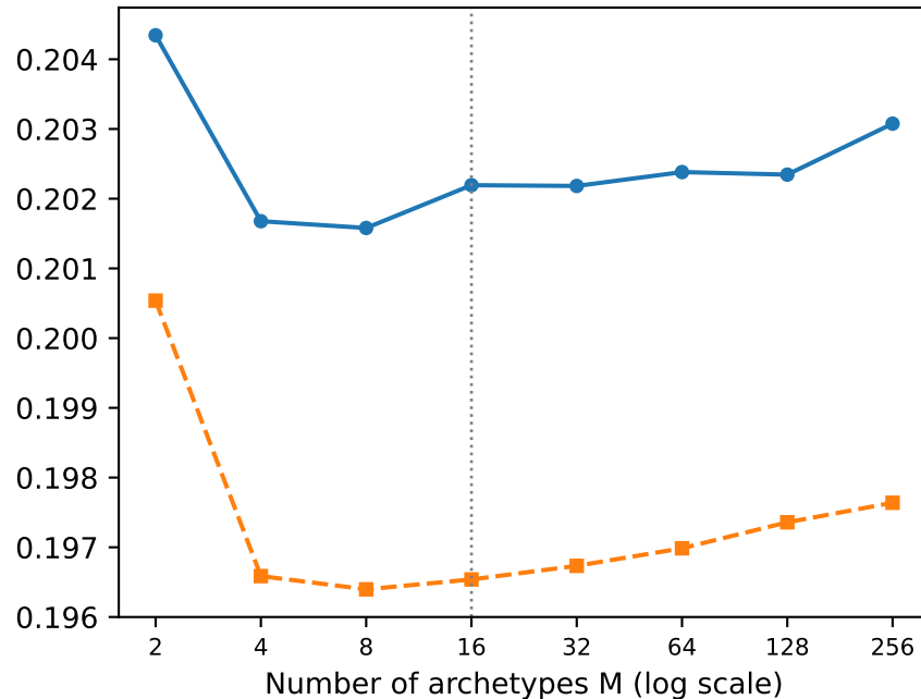
Held-out Brier score
