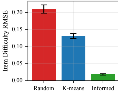
Item Difficulty RMSE
