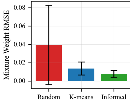
Mixture Weight RMSE
