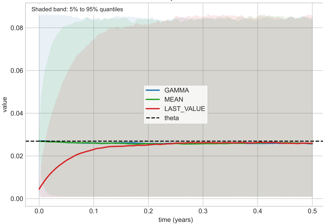
CIR variance trajectories: 6 months
