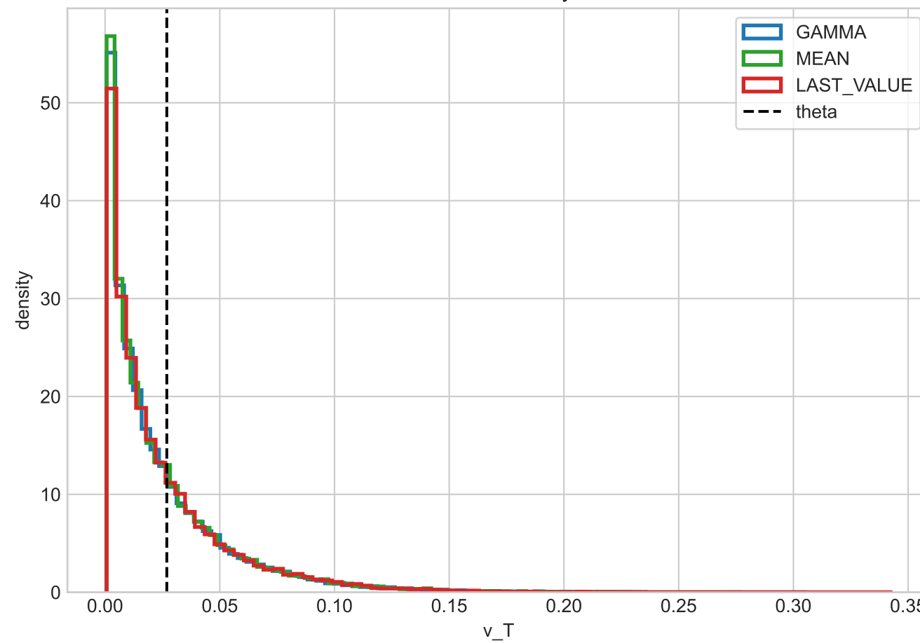
Terminal variance density: 6 months
